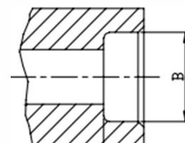
Socket weld bore
