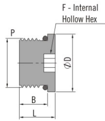
Male SAE/MS Straight Threads
