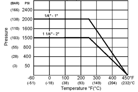
PRESSURE TEMPERATURE RATINGS (BODY)
